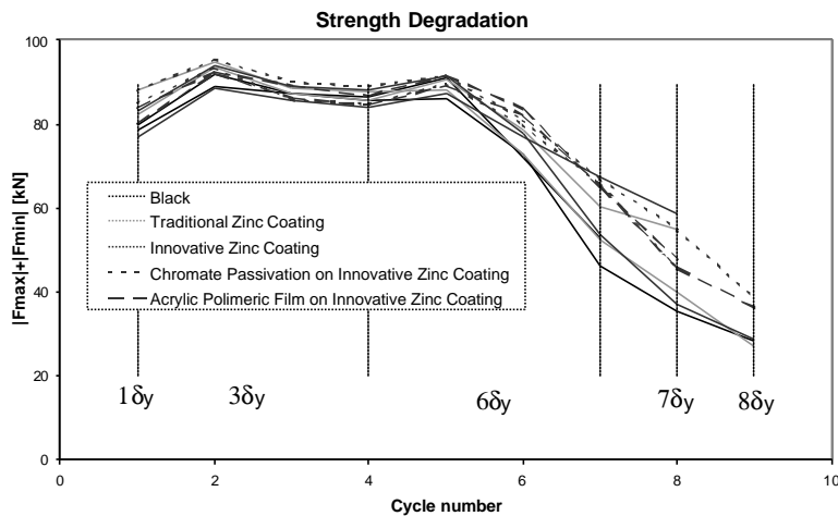
Figure 4: Strength degradation versus the number of cycle as obtained from all the specimens tested.
