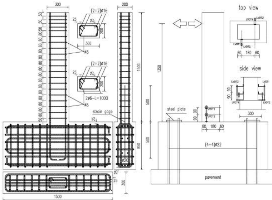
Figure 1: Specimen geometry, reinforcement and instrumentation.
