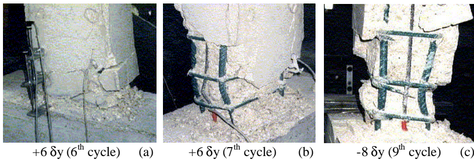
Figure 6: Photographs of the column base as obtained from a specimen (P3) with bars having a thin acrylic polymeric film during (a,b) and at the end of the test (c).
