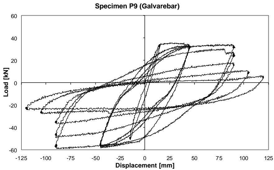
Figure 3: Typical load-displacement relationship as obtained from a specimen (P9) with innovative galvanized steel bars.
