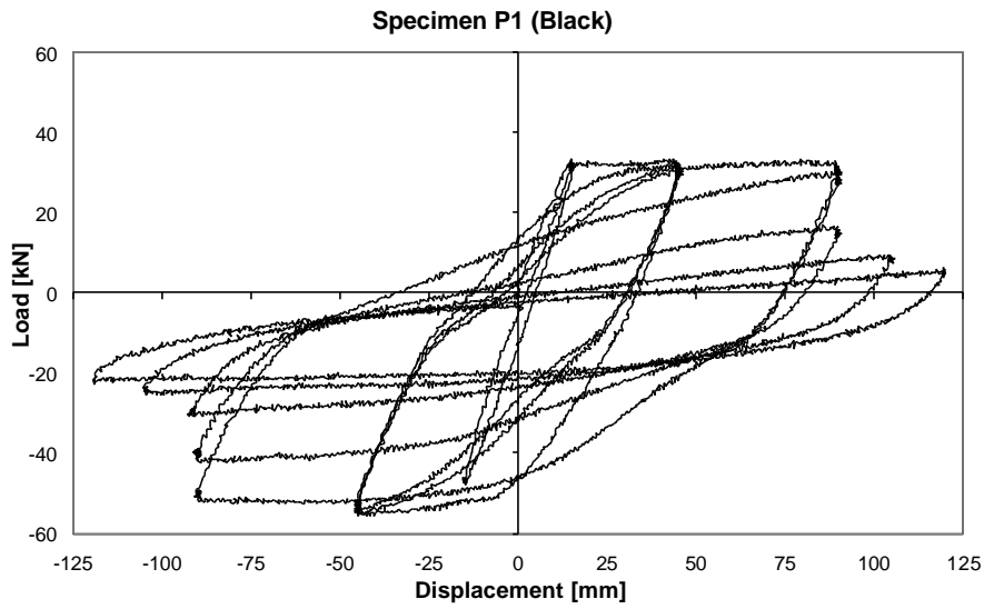
Figure 2: Typical load-displacement relationship as obtained from a specimen (P1) with bars without coating.
