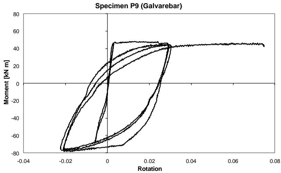
Figure 5: Typical moment-rotation relationship as obtained from a specimen (P9) with innovative galvanized steel bars.
